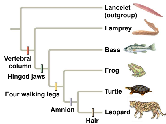
(b) Phylogenetic tree
