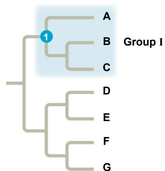
(a) Monophyletic group (clade)
