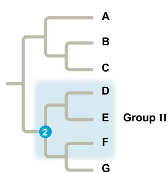
(b) Paraphyletic group
