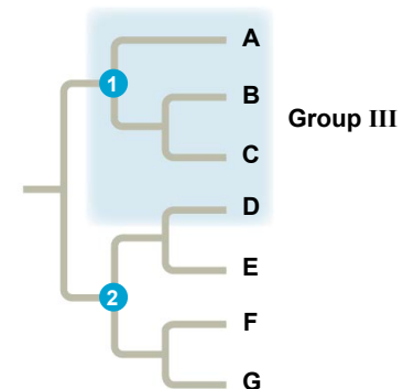
(c) Polyphyletic group
