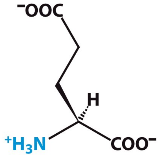
Glutamate
