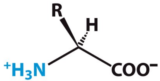
Amino acid
